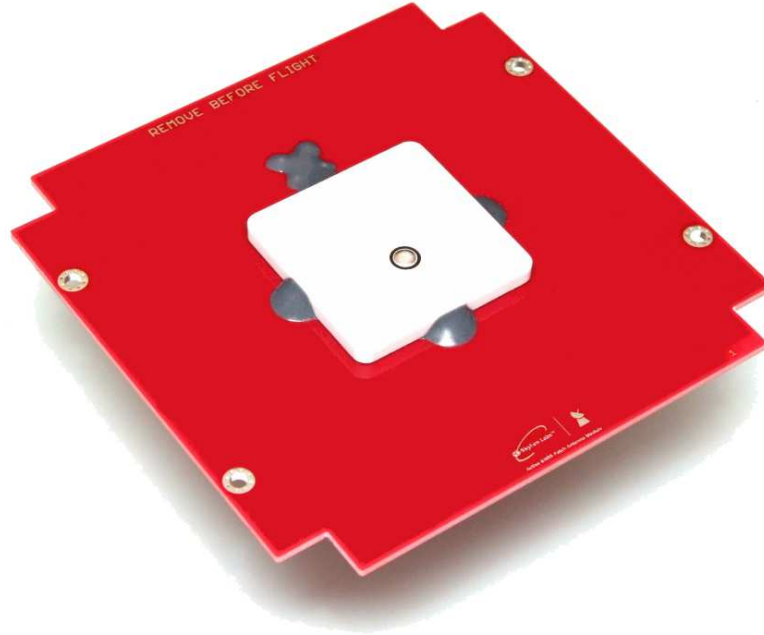
Fig. 3 Engineering Model of the piPATCH-LG unit with red Remove Before Flight finish.
