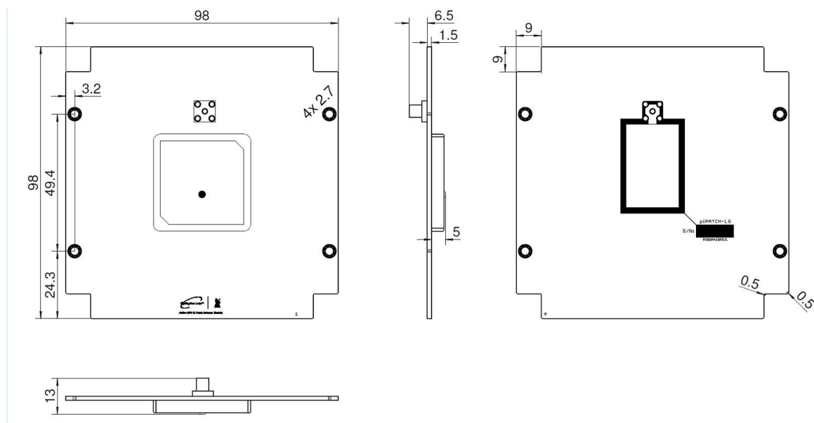
Fig. 2 piPATCH-LG Dimensions drawing, measures are in millimeters. Not to scale.
